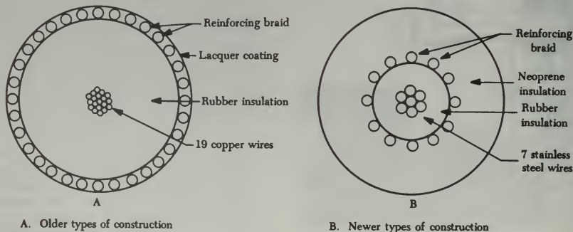
FIGURE 4-68. Cross-sectional view of typical high-tension ignition cable.
